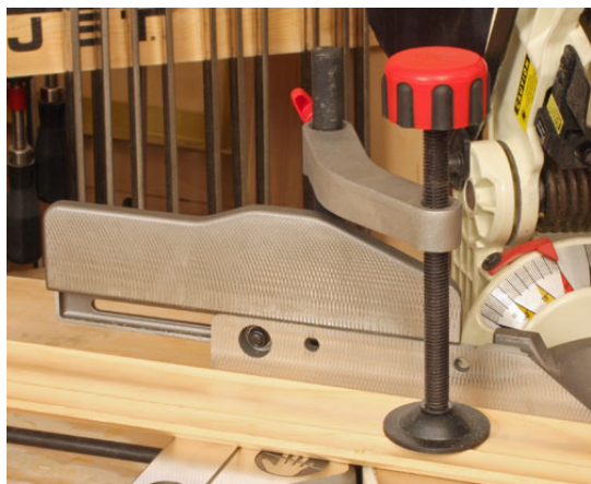
The toll-free work clamp and upper fence section make handling larger pieces of wood more accurate and safer.
